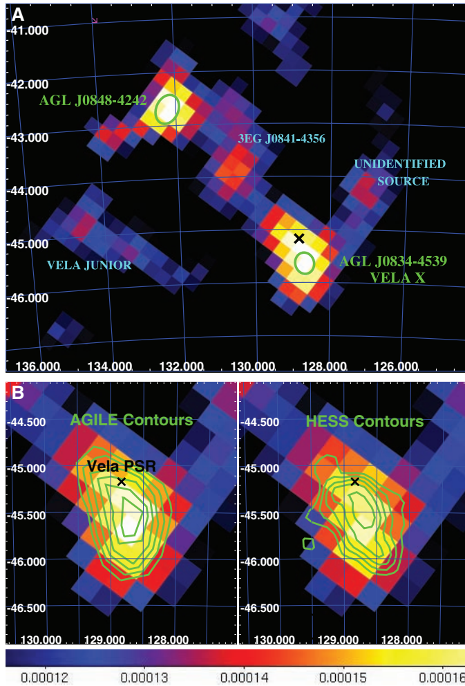
Fig. 1. (A) Gaussian-smoothed AGILE intensity map (photons \text{cm}^{-2} \text{s}^{-1} \text{sr}^{-1} with pixel size 0.25^\circ \times 0.25^\circ ) at E > 400 MeV around the Vela pulsar, including only off-pulse events (i.e., discarding events with phase corresponding to Vela pulsed emission). The neutron star position is marked with a black cross; green circles are the 68% confidence contours for the position of AGL J0848-4242 and AGL J0834-4539 (Vela X). The AGILE E > 400 MeV energy band is well suited for gamma-ray imaging and provides a good compromise between the instrument-effective area ( \sim 400 \text{ cm}^2 ; \sim 100 counts from AGL J0834-4539) and point-spread function ( \sim 1^\circ , 68% containment radius), both parameters decreasing with energy. (B) The gamma-ray diffuse source AGL J0834-4539. AGILE contours (left) are in the range 1.4 \times 10^{-4} to 1.6 \times 10^{-4} photons \text{cm}^{-2} \text{s}^{-1} \text{sr}^{-1} , with step 4 \times 10^{-6} . HESS contours (right) are from (10).
